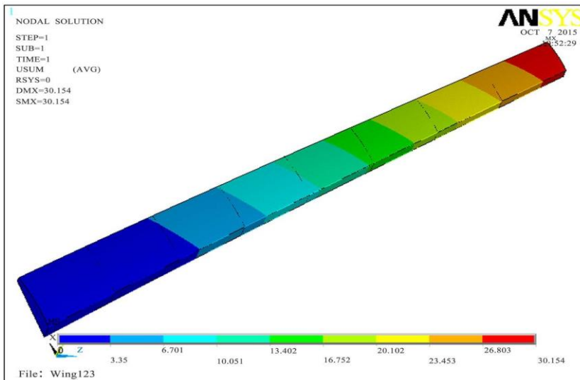
Figure 16. Strain cloud map.
