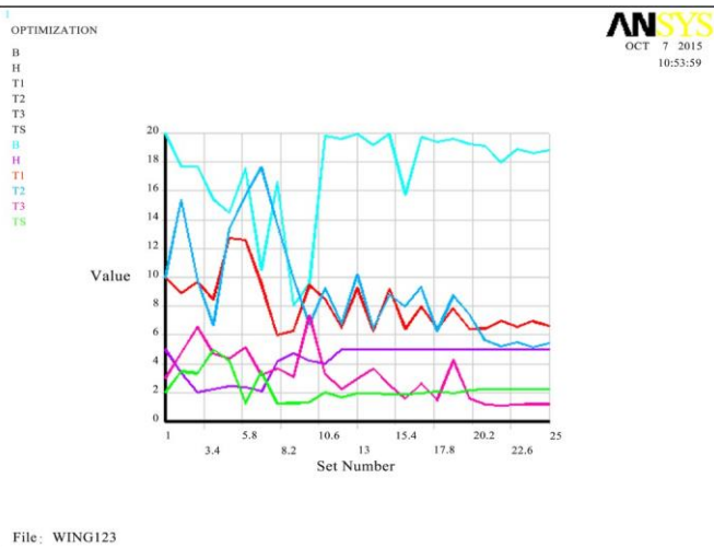
Figure 13. Geometric parameter change during optimization.
