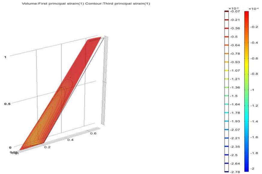
Figure 10. Third principle strain cloud map.
