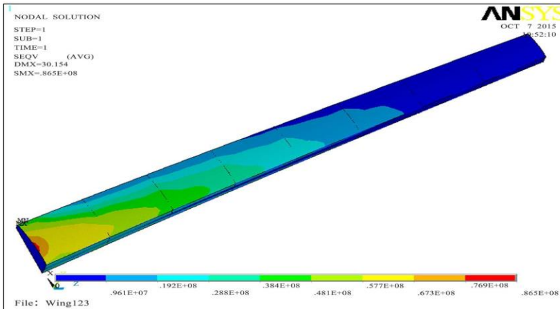
Figure 15. Stress cloud map.
