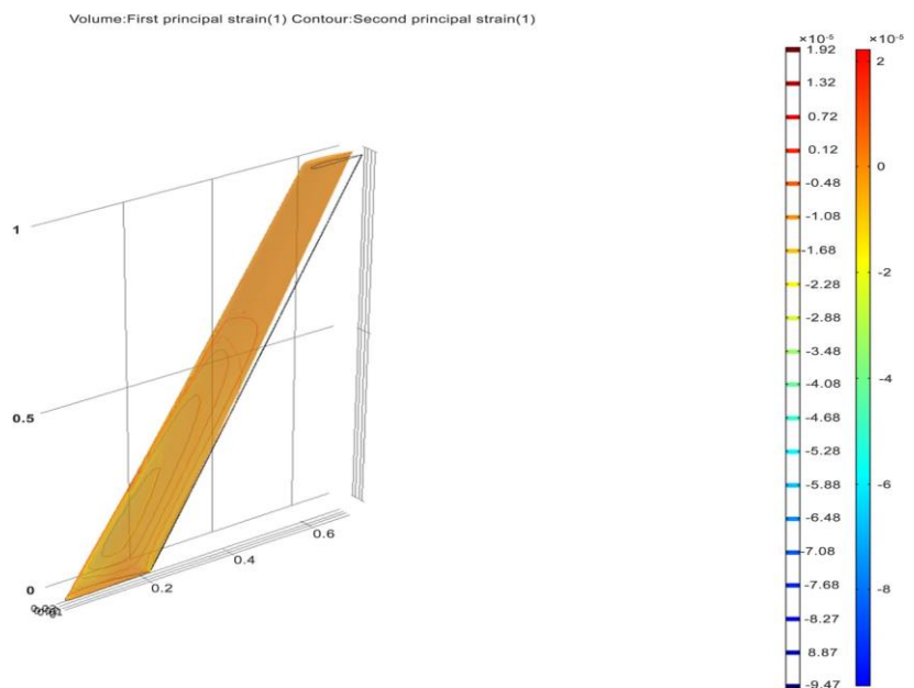
Figure 9. Second principle strain cloud map.
