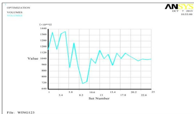
Figure 14. Volume change during optimization.
