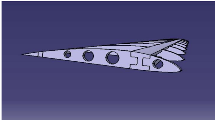
Figure 17. Overall wing structure form.
