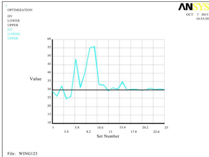
Figure 12. Deflection change during optimization.
