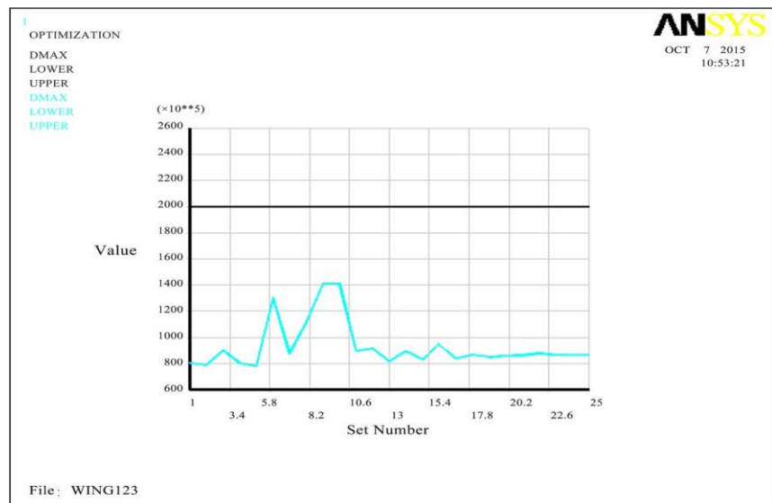
Figure 11. Stress change during optimization.
